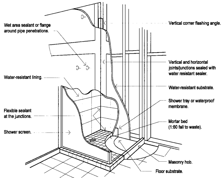
Figure 3.8.1.5 TYPICAL VIEW OF SHOWER RECESS AND LINING MATERIALS
