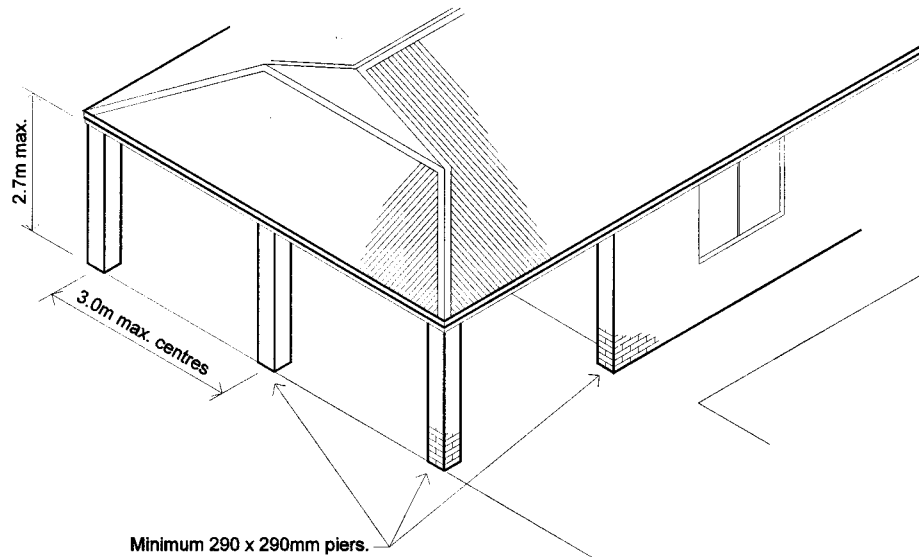
Figure 3.3.1.5 ISOLATED PIERS UNDER MAIN ROOF
