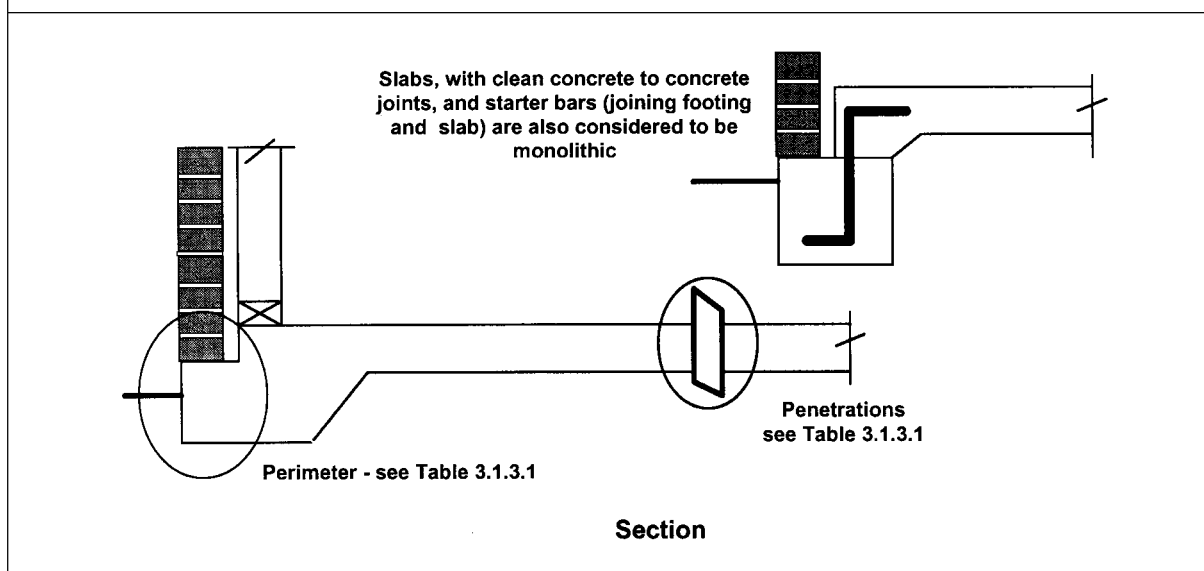
Figure 3.1.3.2 AREAS TO BE PROTECTED FOR MONOLITHIC SLABS
