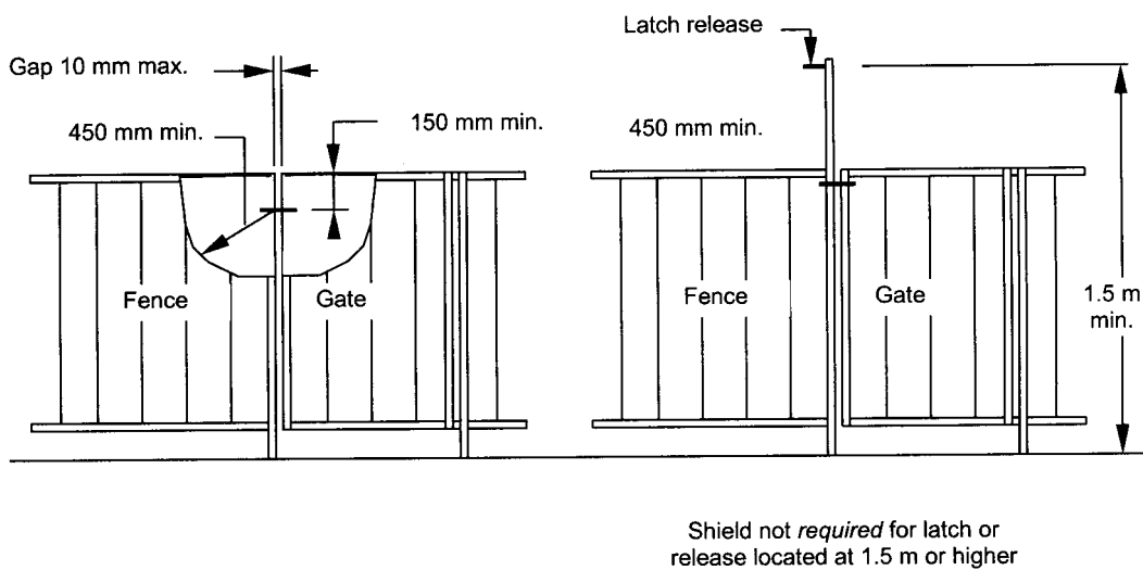
Figure 3.9.3.7 LOCATION AND SHIELDING OF GATE LATCHES
