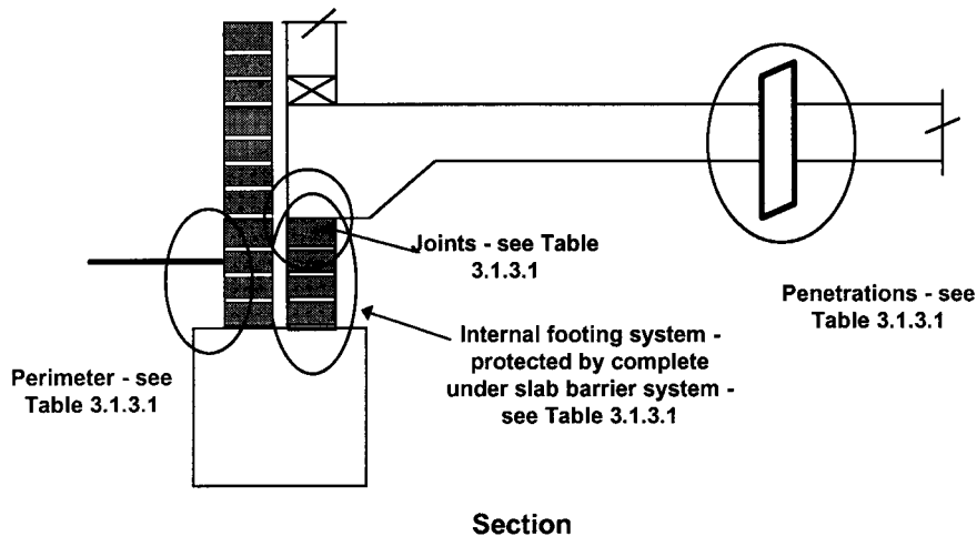
Figure 3.1.3.3 AREAS TO BE PROTECTED FOR NON-MONOLITHIC SLABS
