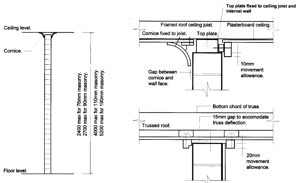
Figure 3.3.1.4 SUPPORT FOR INTERNAL WALLS (Dimensions in mm)
