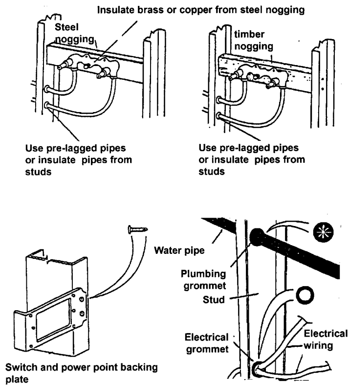
Figure 3.4.2.7 TYPICAL INSTALLATION AND FIXING OF SERVICES
