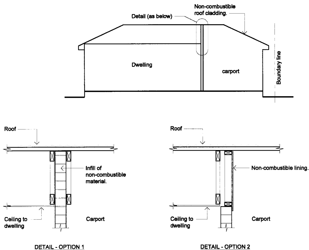
Figure 3.7.1.8 REQUIREMENTS FOR NON-COMBUSTIBLE INFILL PANELS TO CARPORT
