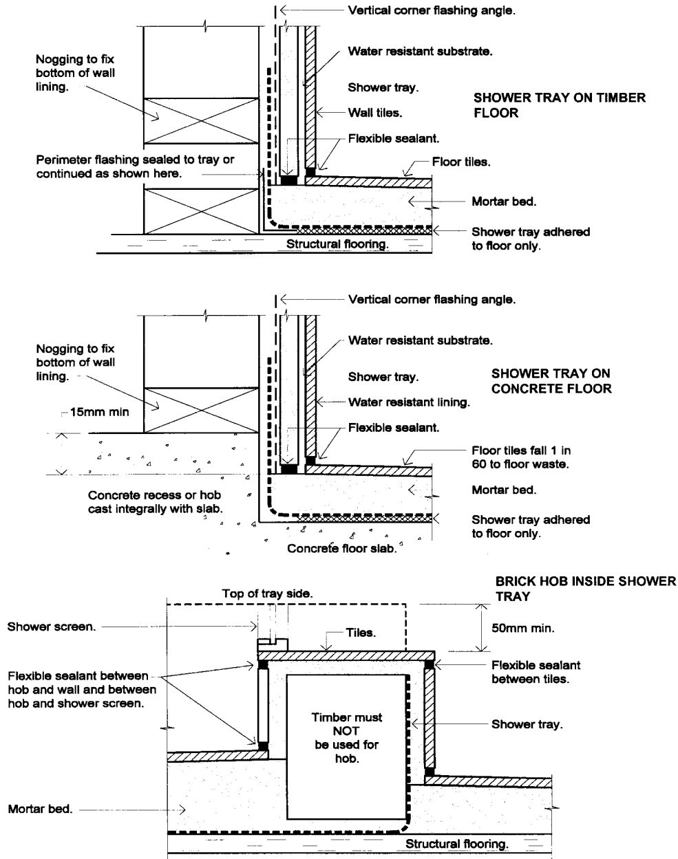
Figure 3.8.1.8 FLOORS IN SHOWER AREAS
