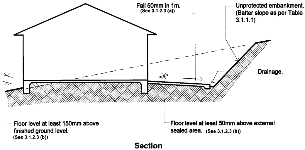
Figure 3.1.2.2 SITE SURFACE DRAINAGE
