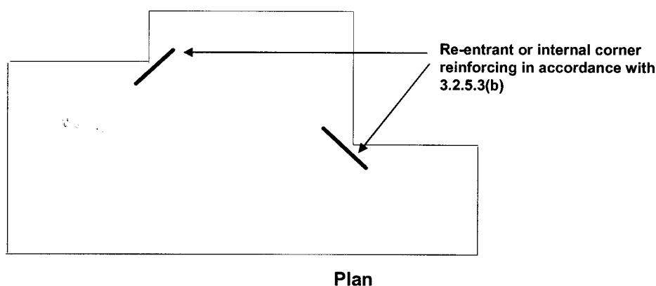
Figure 3.2.5.1 REINFORCING AT RE-ENTRANT CORNERS
