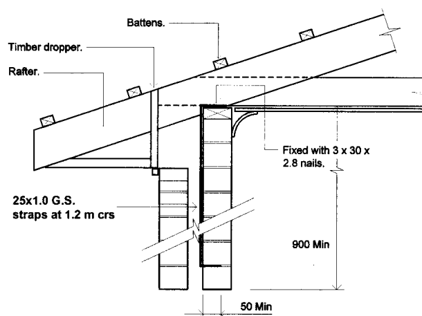
Figure 3.3.3.3 SUITABLE TIE DOWN STRAP DETAILS
