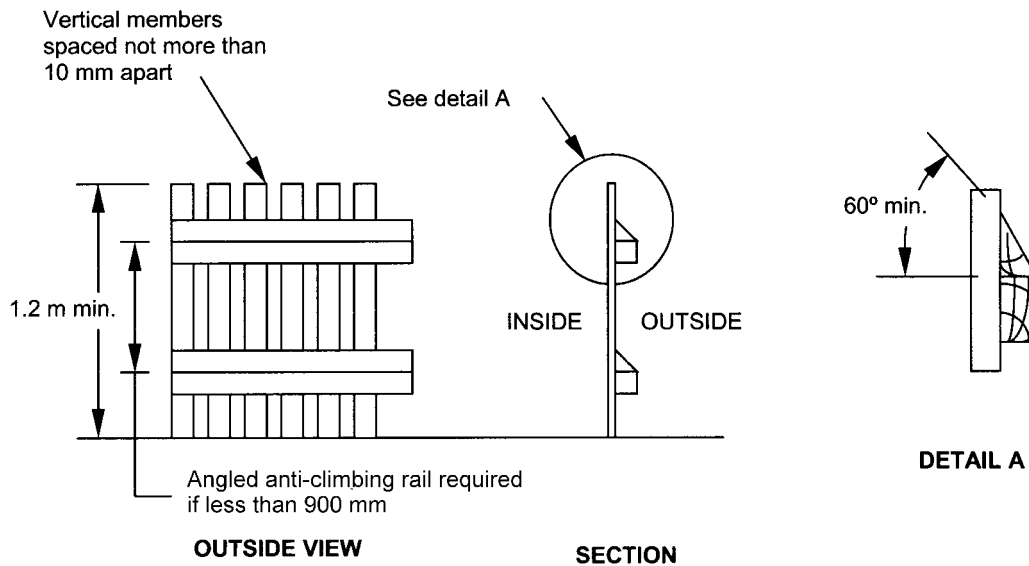
Figure 3.9.3.6 HORIZONTAL MEMBERS NOT ACTING AS A HOLD FOR CLIMBING
