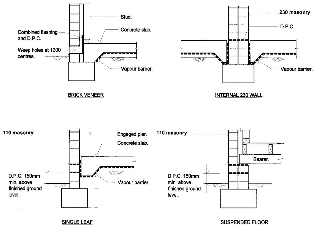
Figure 3.3.4.4 CORRECT INSTALLATION OF DPC IN SUB-FLOOR STRUCTURES
