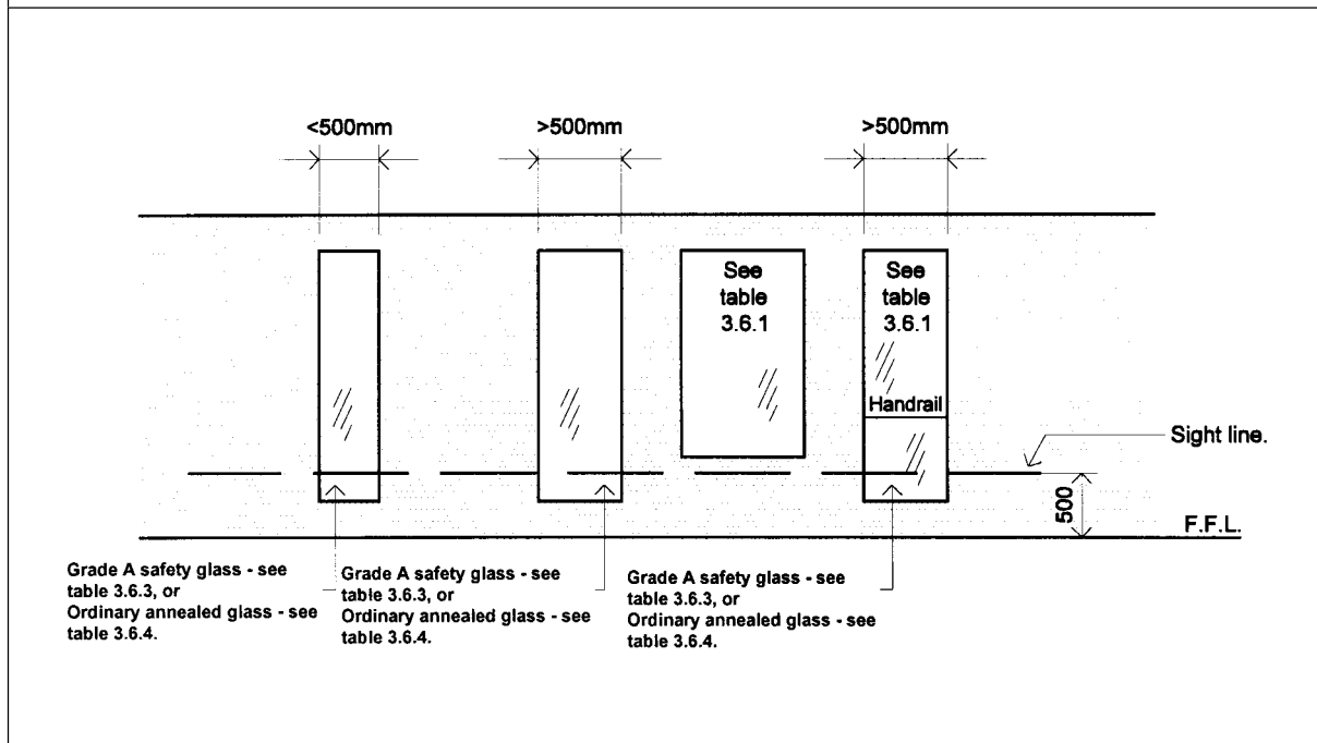
Figure 3.6.2 IDENTIFICATION OF GLAZING REQUIREMENTS FOR GLAZED PANELS
