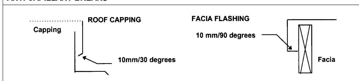
Figure 3.5.1.6 ANTI CAPILLARY BREAKS
