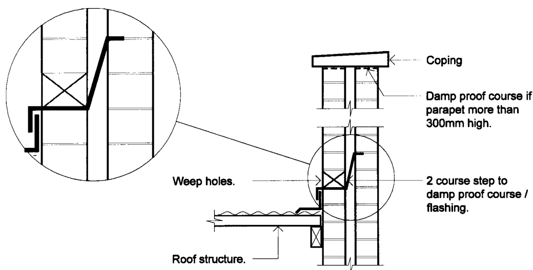
Figure 3.3.4.2 INSTALLATION OF DPCs FOR PARAPET WALLS
