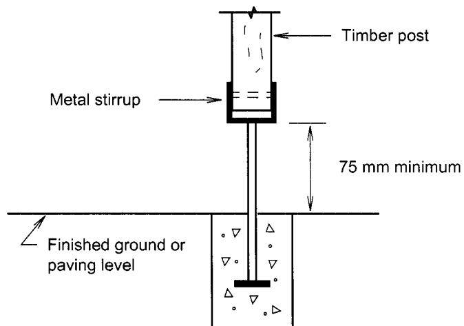
Figure 3.7.4.2 METAL STIRRUP CLEARANCE
