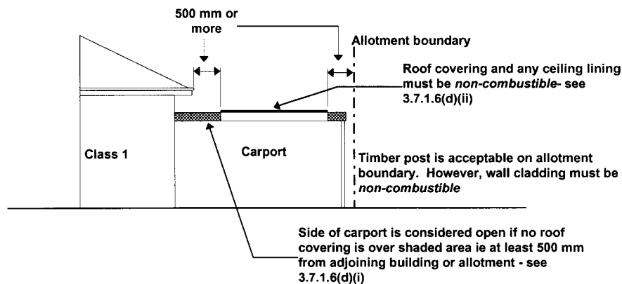
Figure 3.7.1.7 IDENTIFYING AN OPEN CARPORT
