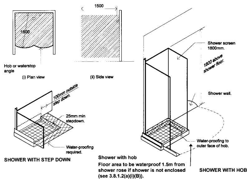
Figure 3.8.1.1 ENCLOSED AND UNENCLOSED SHOWER – AREA TO BE PROTECTED
