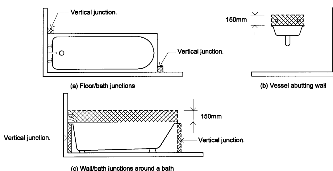
Figure 3.8.1.3 BATH AND WALL FIXTURES – AREA TO BE PROTECTED
