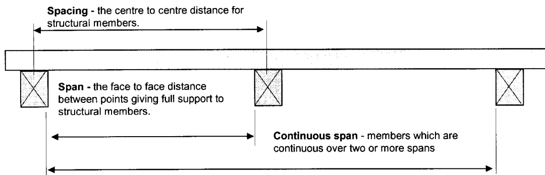
Figure 3.4.0.1 SPAN AND SPACING TERMS
