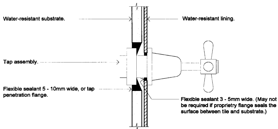
Figure 3.8.1.6 TYPICAL INSTALLATION OF TAP FLANGE
