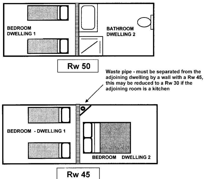
Figure 3.8.6.1 REQUIRED R_w – PLAN VIEW
