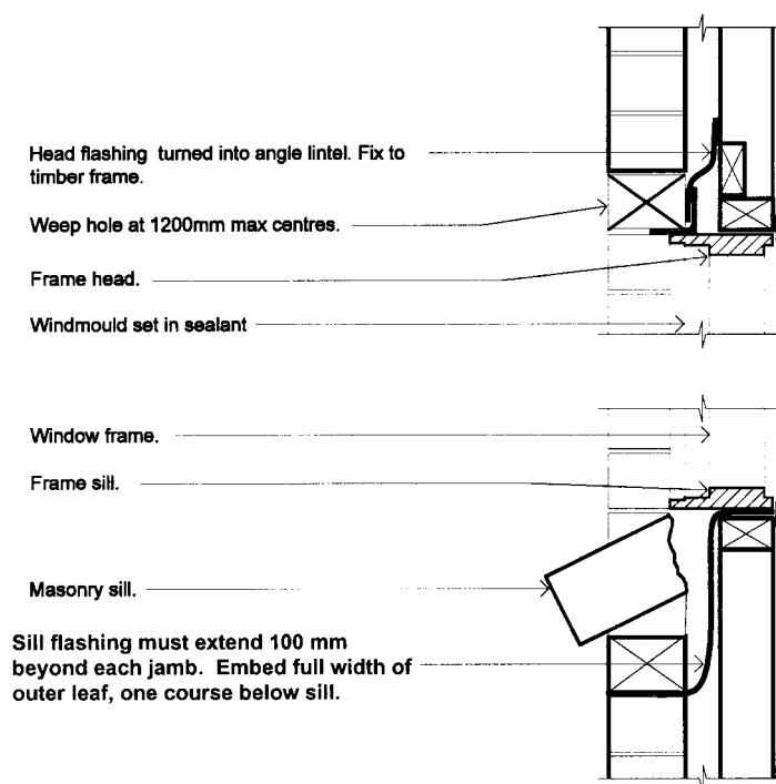
Figure 3.3.4.6 FLASHING OF OPENINGS IN MASONRY VENEER WALLS
