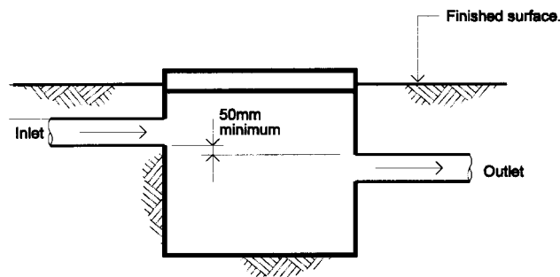
Figure 3.1.2.4 CONSTRUCTION OF SILT PITS
