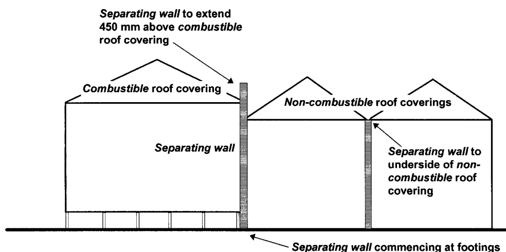
Figure 3.7.1.10 SEPARATING WALL CONSTRUCTION
