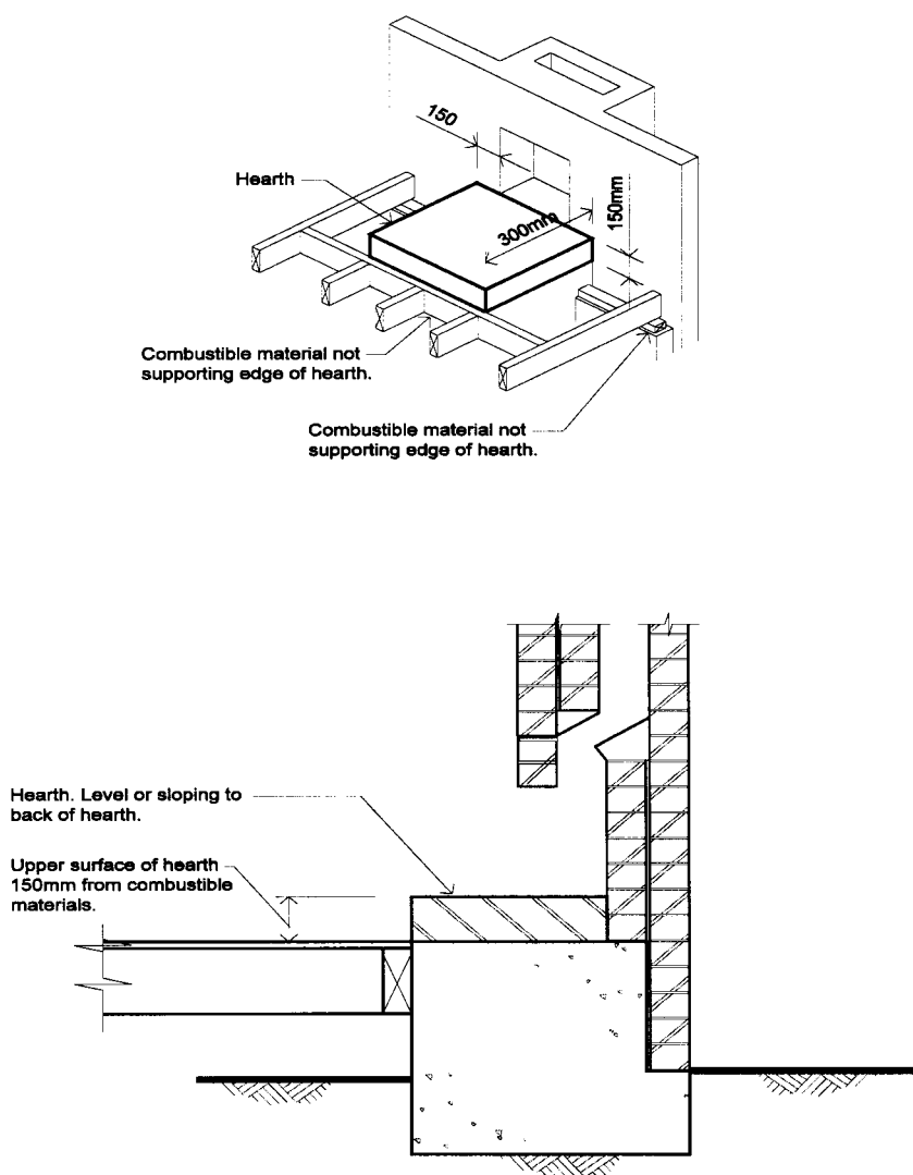
Figure 3.7.3.1 FIRE PLACE CLEARANCE FROM COMBUSTIBLE MATERIALS
