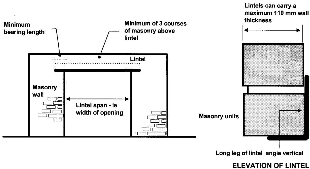
Figure 3.3.3.4 LINTEL INSTALLATION
