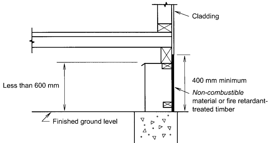
Figure 3.7.4.1 PROTECTION OF SUB-FLOOR SPACES WITH LESS THAN 600 MM CLEARANCE
