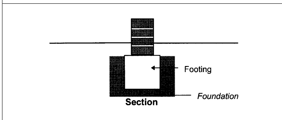
Figure 1.1.2 IDENTIFICATION OF FOUNDATION
