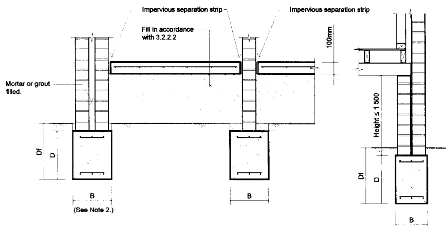
DIMENSIONS AND REINFORCEMENT FOR STRIP FOOTING SYSTEMS
