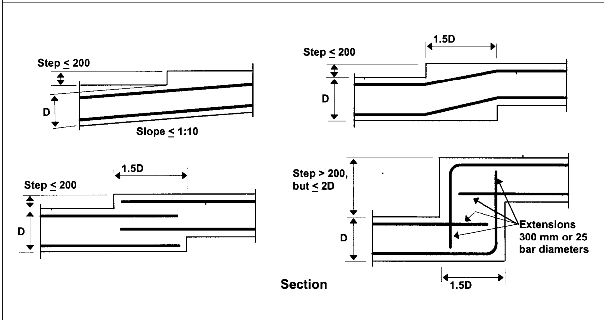
Figure 3.2.2.2 STEPPED STRIP FOOTINGS
