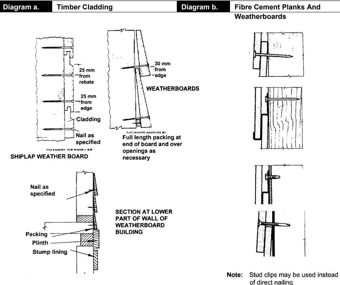
Figure 3.5.3.1 FIXING OF WALL CLADDING
