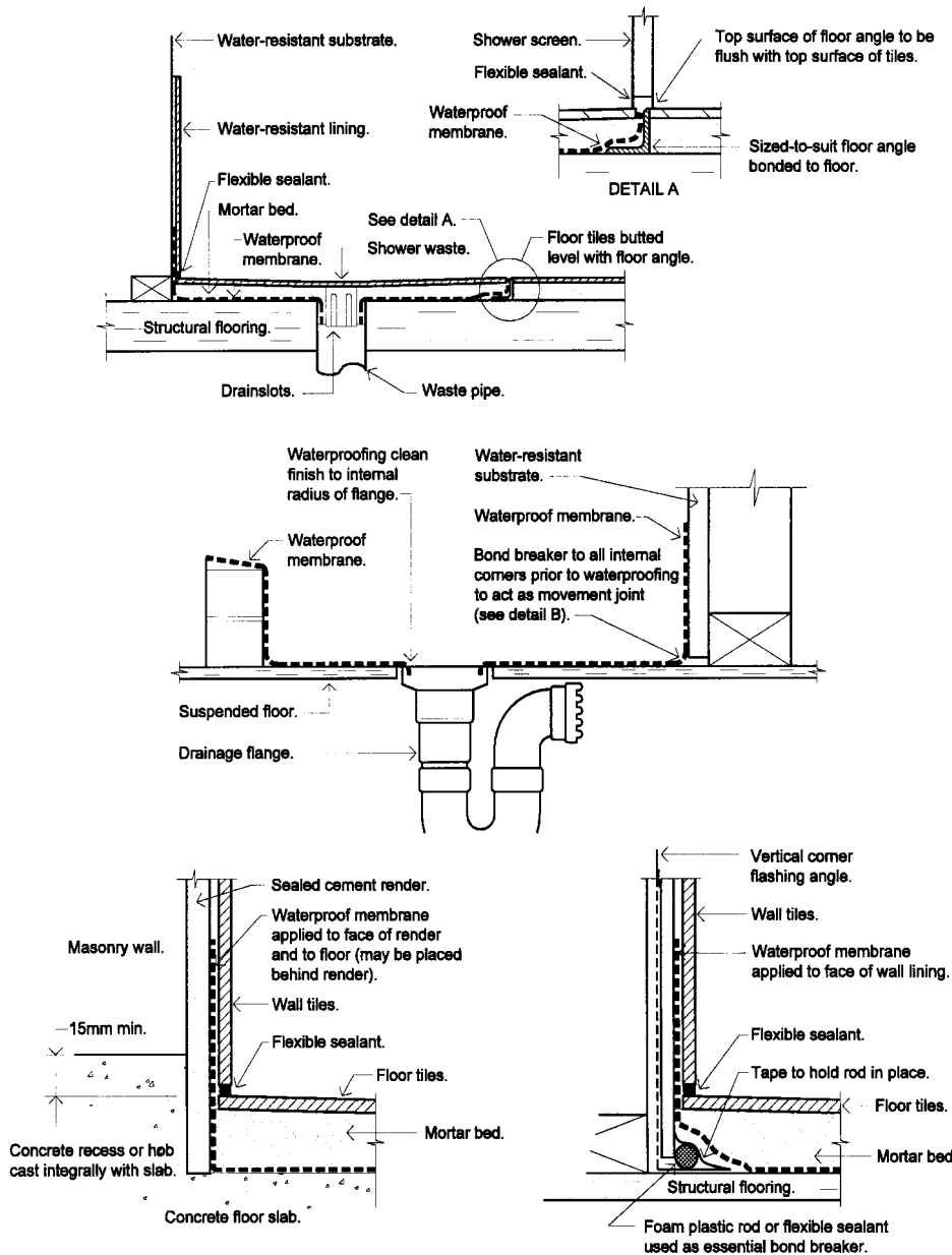
Figure 3.8.1.9 TYPICAL INSTALLATION OF WATERPROOF MEMBRANE TO SHOWER FLOOR
